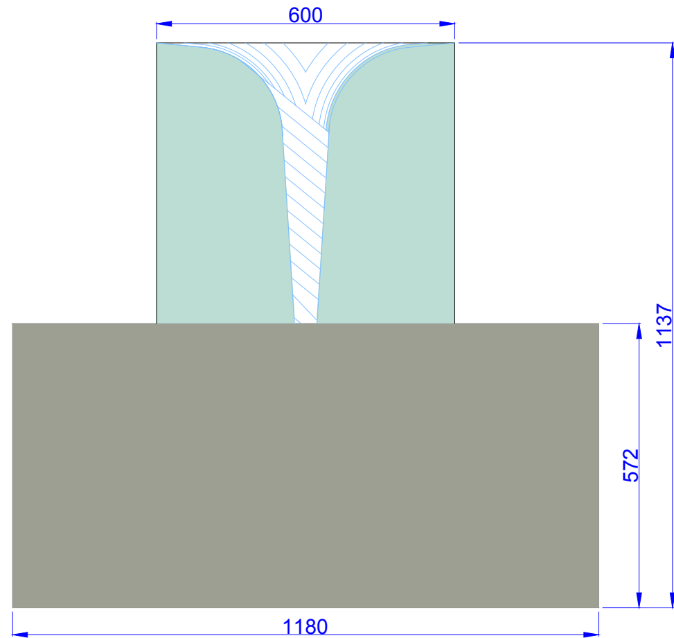
FRONT ELEVATION
