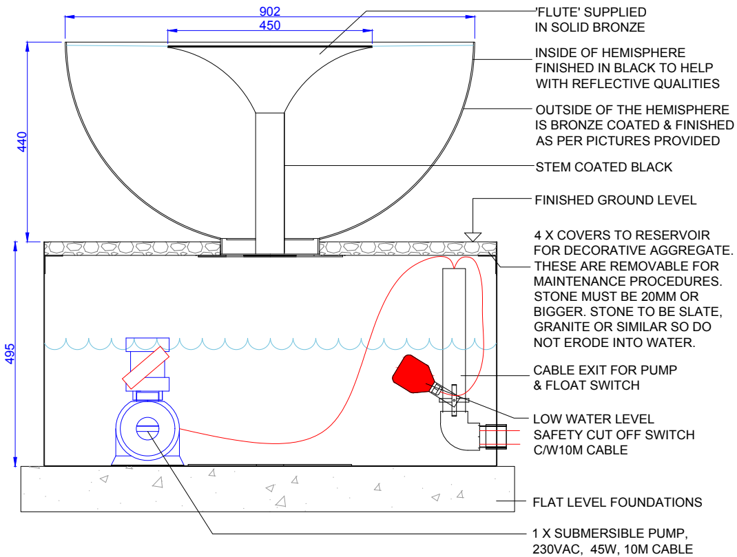
TYPICAL SECTION VIEW
