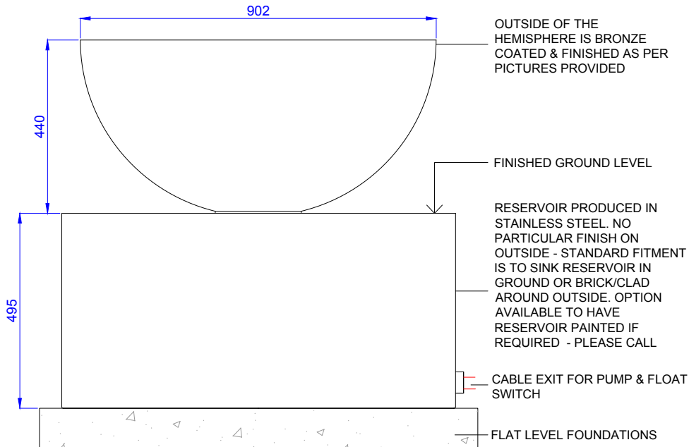
SIDE VIEW
